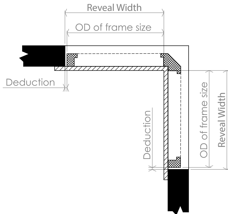
L-FRAME CORNER POST REVEAL FIT
